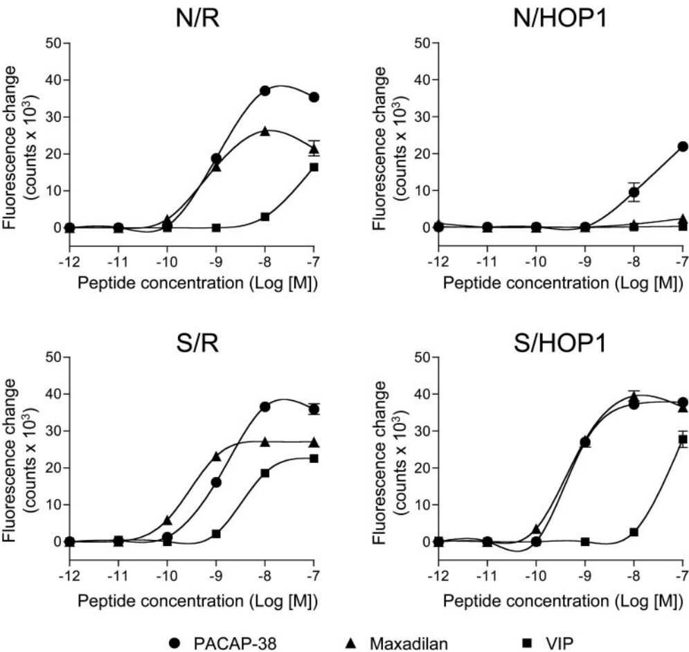
Fig. 5. Effects of PACAP-38, VIP, and maxadilan on the increase in the [Ca 2+ ] i in CHO cells stably expressing the PAC1 isoforms. After incubating the cells with a fluorescent indicator dye at 37°C for 1 h, changes in the [Ca 2+ ] i were assayed using a fluorometric imaging plate reader with various concentrations of the agonists. ●, PACAP-38; ▲, maxadilan; ■, VIP.
