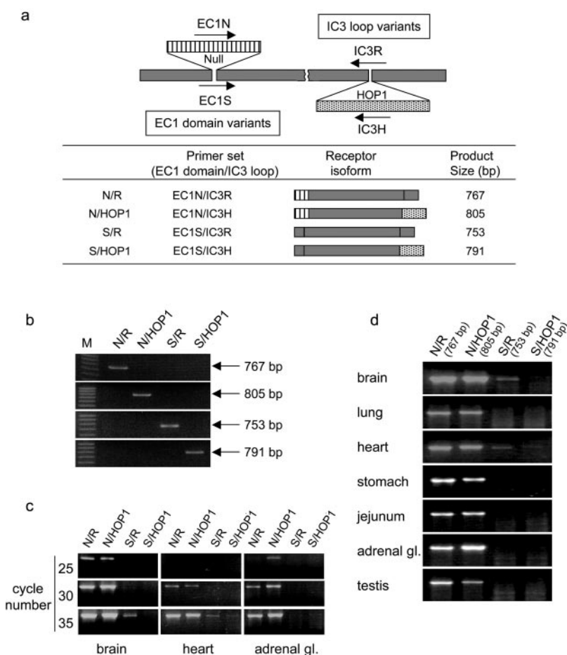
Fig. 1. Expression of the PAC1 isoforms in mouse tissues. a, schematic diagrams of the PAC1 isoforms. PAC1 isoforms that differ in either the EC1 domain and/or the IC3 loop are created by alternative splicings. As indicated, four primers were designed to allow us to specifically amplify each of the four potential isoforms. b, PCR analysis of the plasmids used to create cell lines that stably expressed each of the PAC1 isoforms. The PCRs were performed using isoform-specific primer sets. The amplified PCR products containing the regions coding for the EC1 domain and the IC3 loop were detected as single bands. The 805-, 791-, 767-, and 753-bp amplification products correspond to the N/HOP1, S/HOP1, N/R, and S/R isoforms, respectively. c, the linear range of amplifications of the four PAC1 isoforms were verified by varying the number of PCR cycles (25, 30, and 35) in brain, heart, and adrenal gland. d, tissue distributions of the splice variants in mouse tissues. cDNA from each mouse tissue was amplified using oligonucleotide primer sets that specifically amplified each isoform.
